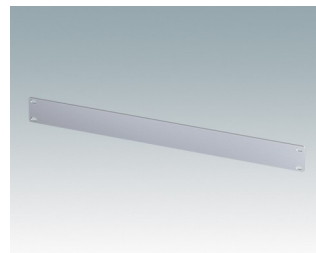
M6019010 Frontplatte 1HEx19" Aluminium Matt eloxiert 482,6x3x43,6mm
